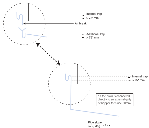
Figure 20: Condensate trap options
