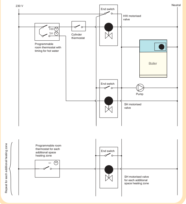
Figure 12: Boiler interlock in a system with two, 2-port valves (this shows the general logic and should not be interpreted as an installation instruction, as the actual wiring will depend on the particular products used).
