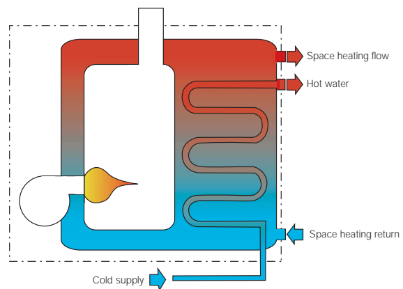
Figure 3: Combi boiler
