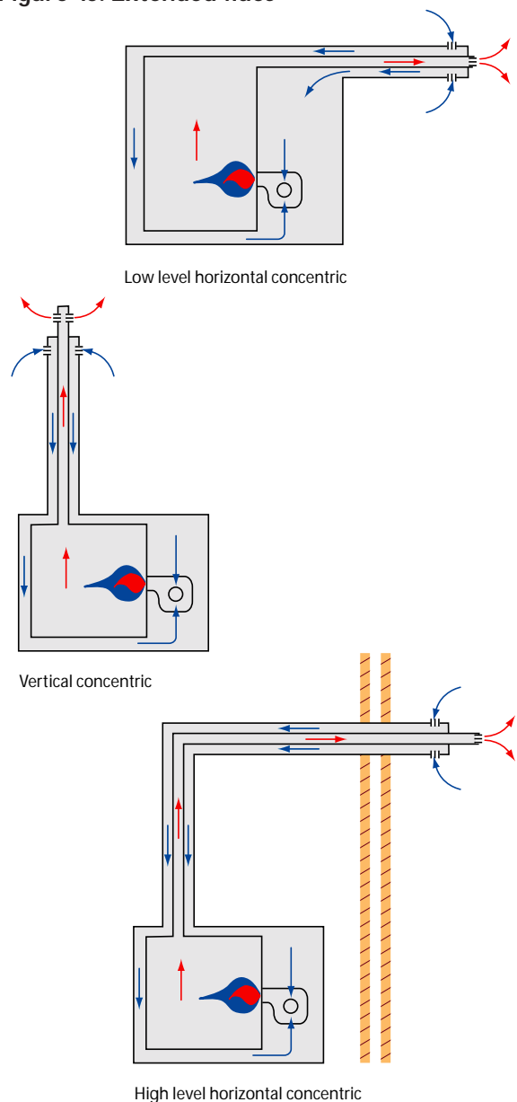
Figure 10: Extended flues
