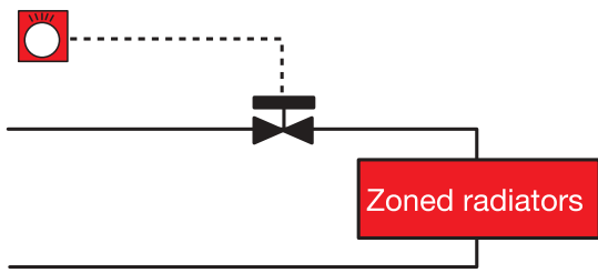
Figure 15: Zone controls
